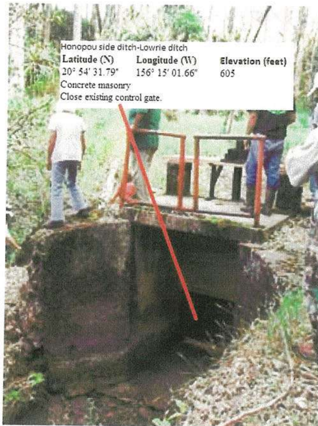
Photo 3 (above): Control gate on Honopou at Lowrie Ditch (L-17) Photo 4 (below): Sluice gate on Honopou at Lowrie Ditch (L-17)
