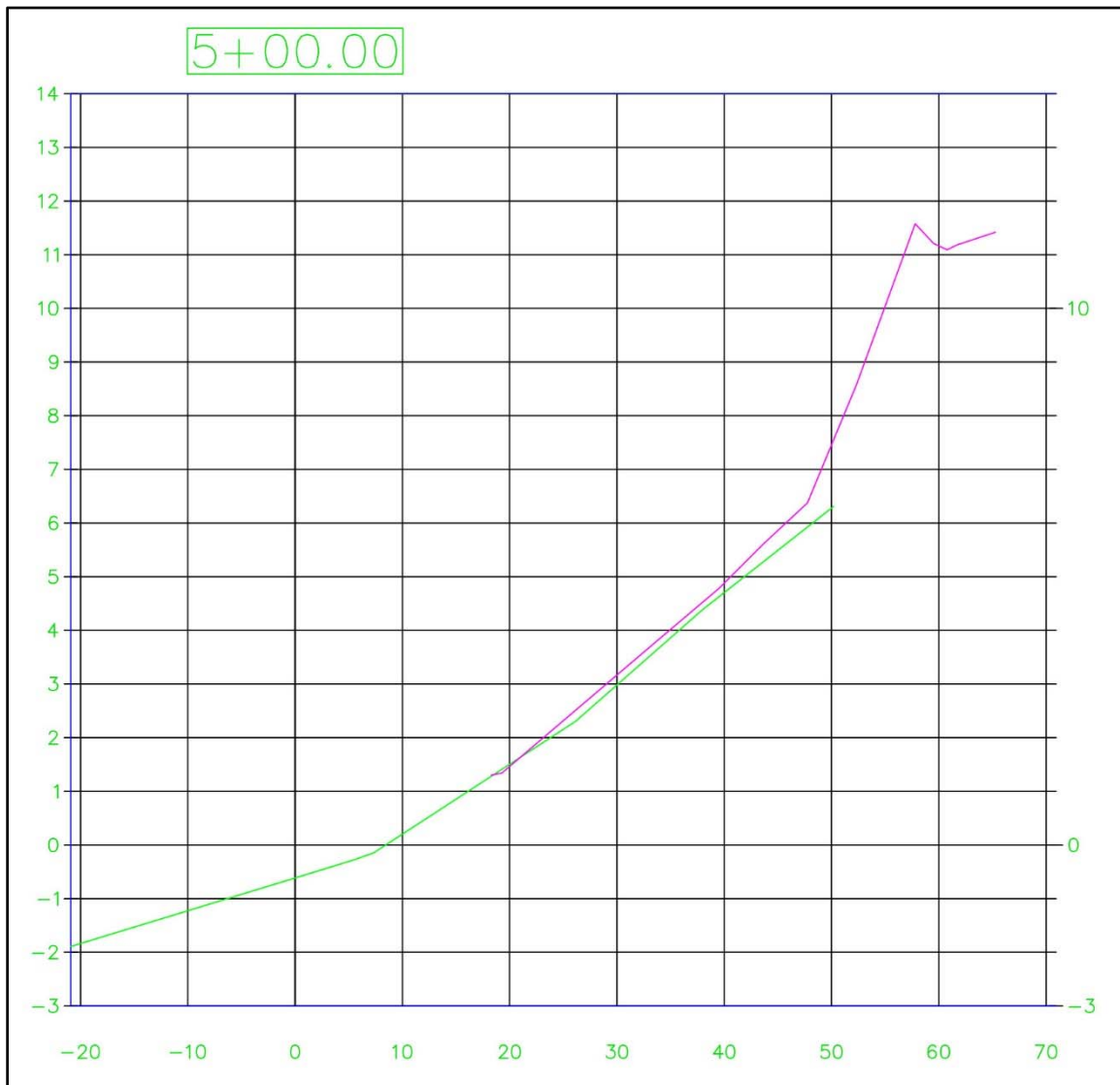
Figure 5-27 Profile 5 + 00. Green and pink lines represent November 09, 2015, and November 10, 2015, elevations respectively.
