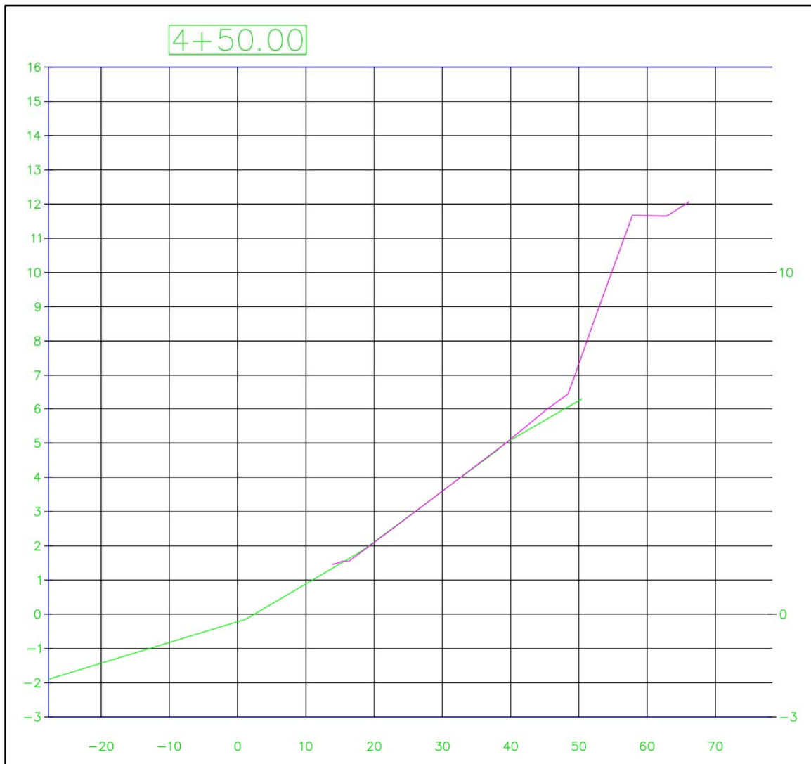
Figure 5-26 Profile 4 + 50. Green and pink lines represent November 09, 2015, and November 10, 2015, elevations respectively.
