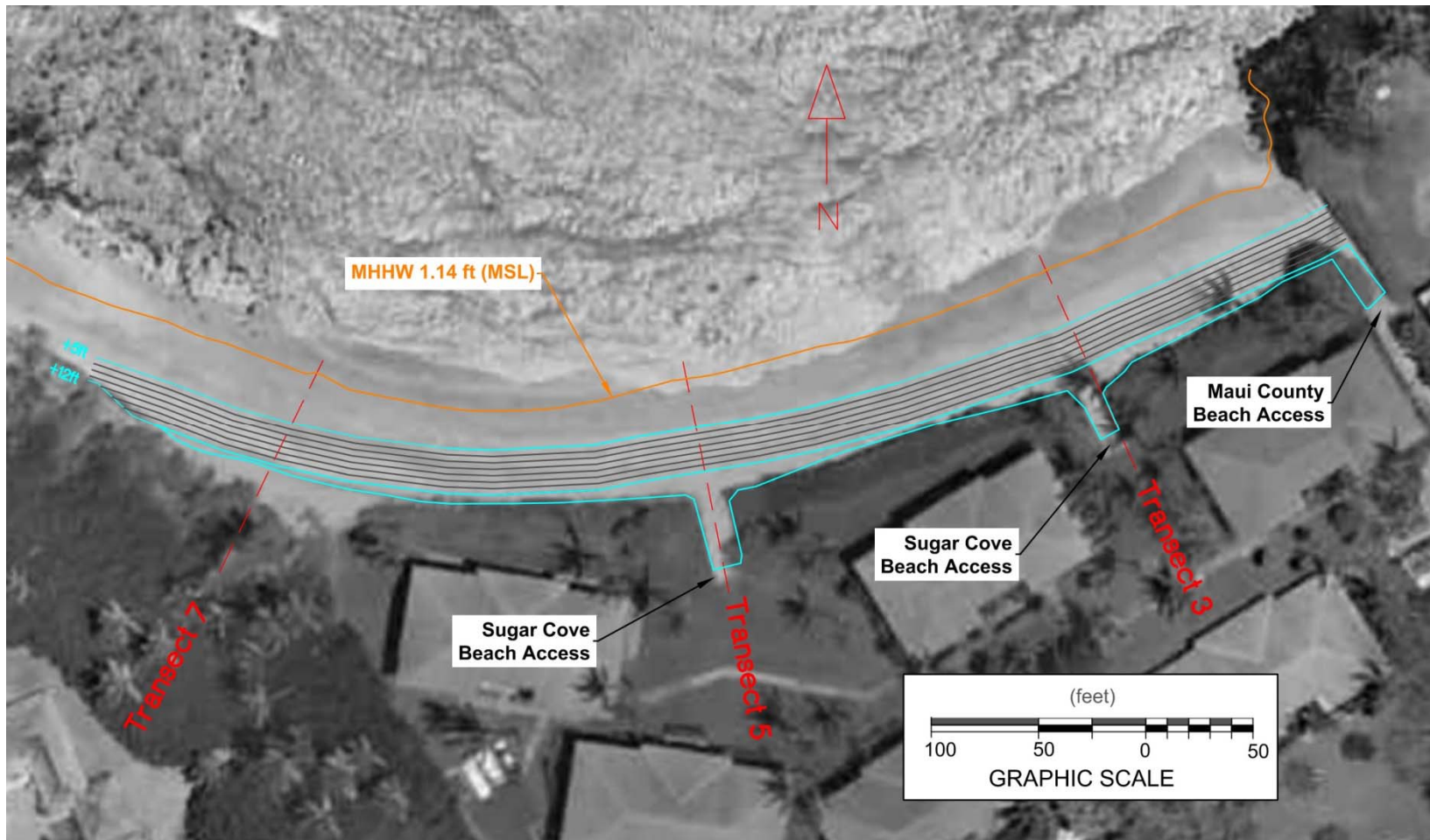
Figure 2-1 Proposed berm maintenance location and contours (LMSL Datum)
