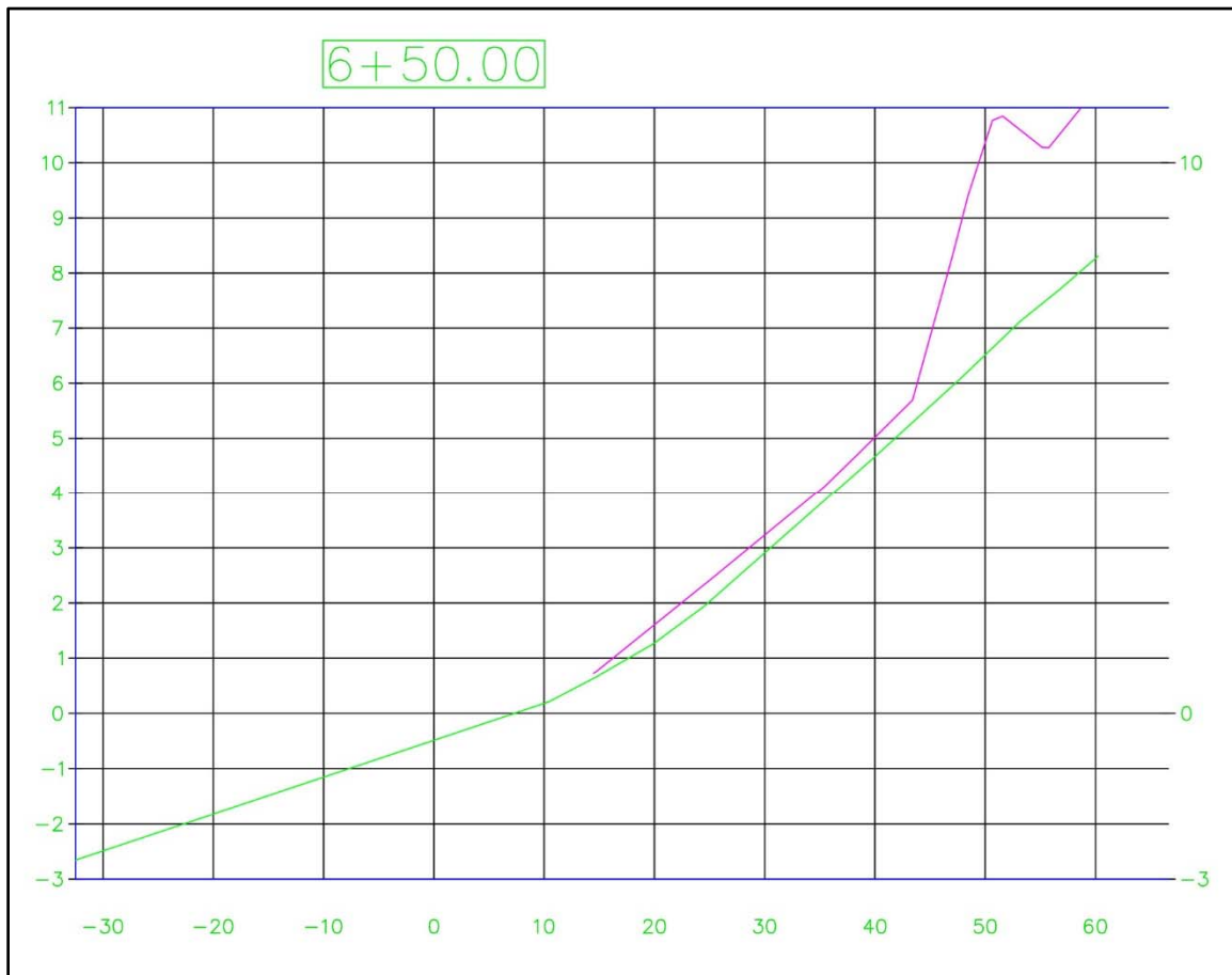
Figure 5-30 Profile 6 + 50. Green and pink lines represent November 09, 2015, and November 10, 2015, elevations respectively.
