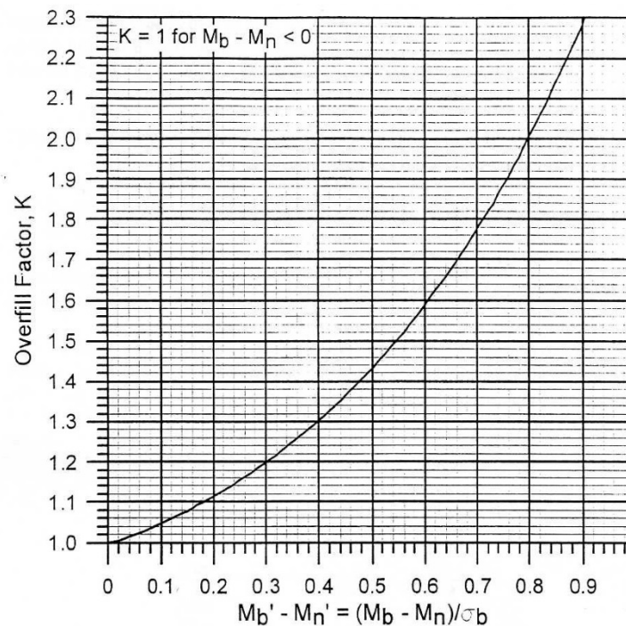
Figure 5-5 Overfill Factor conversion chart
