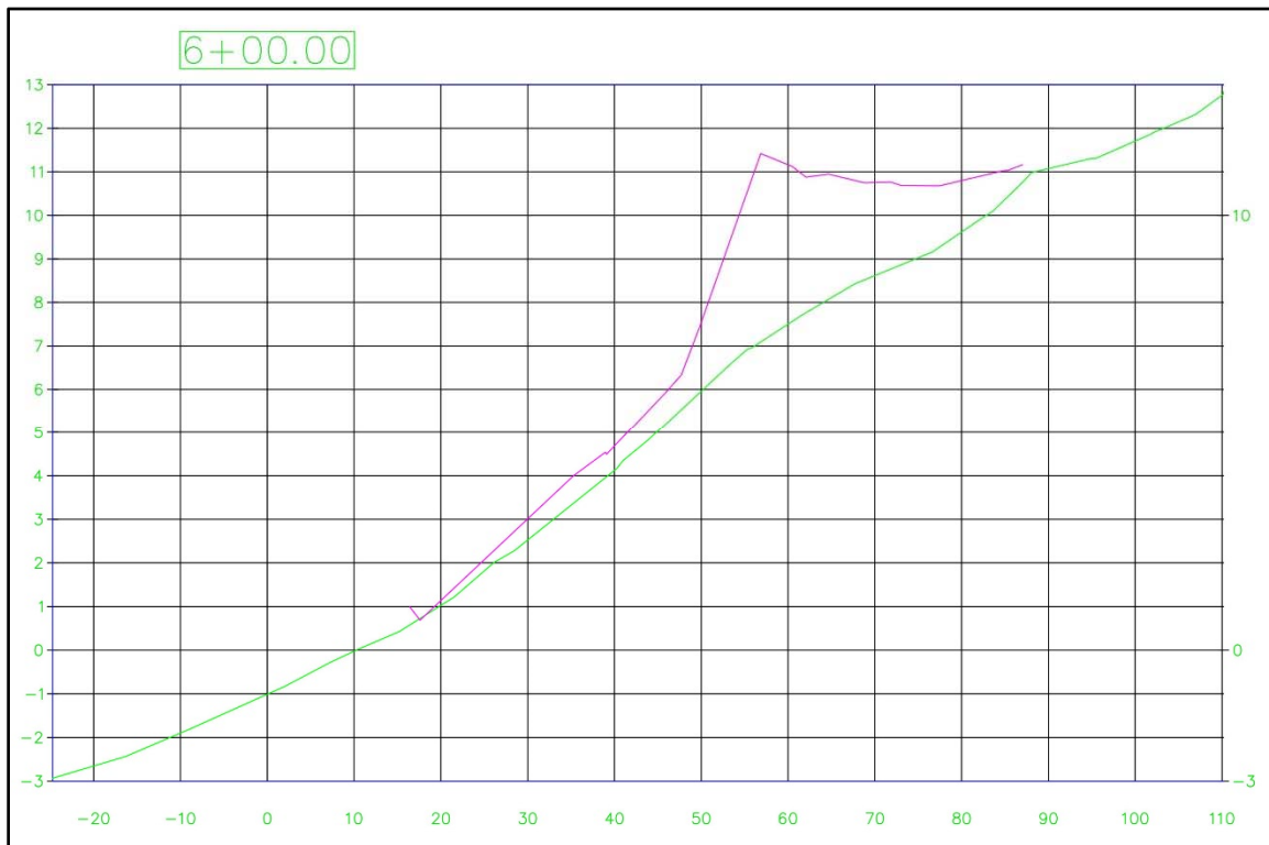
Figure 5-29 Profile 6 + 00. Green and pink lines represent November 09, 2015, and November 10, 2015, elevations respectively.
