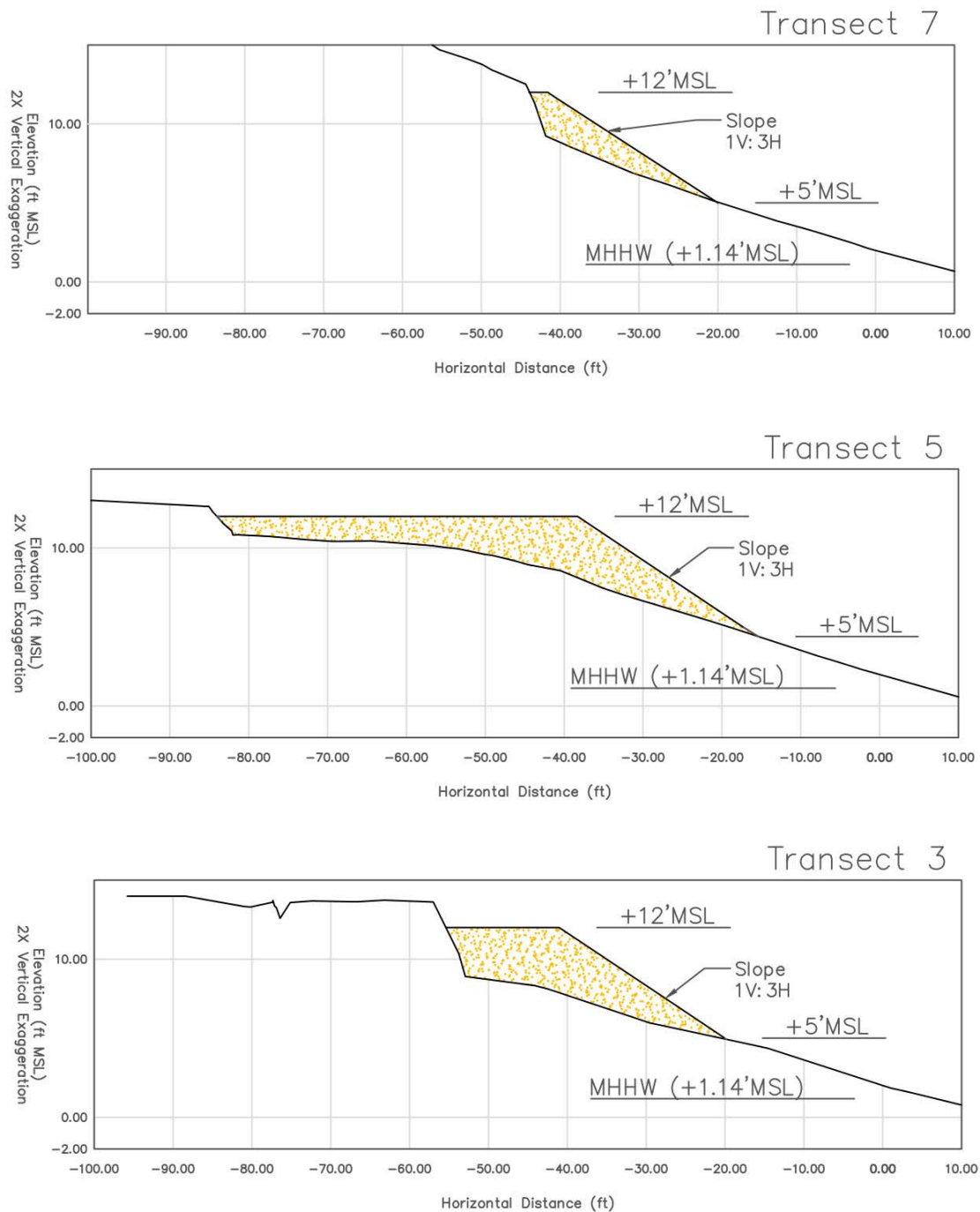
Figure 2-2 Proposed berm maintenance profiles (LMSL Datum)
