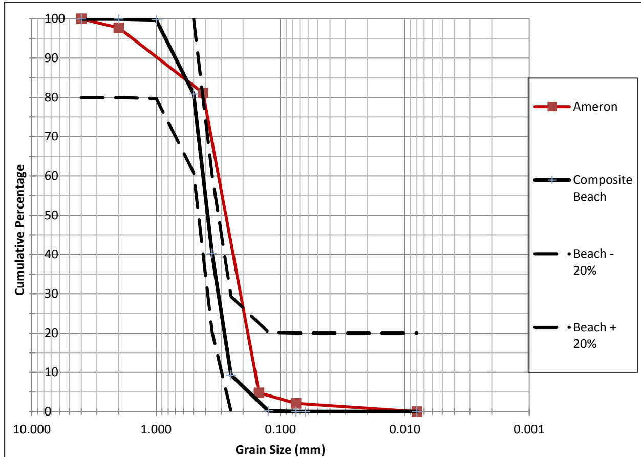
Figure 5-4 Grain size distribution for composite beach sample, the +/- 20% thresholds, and the berm fill sand sample
