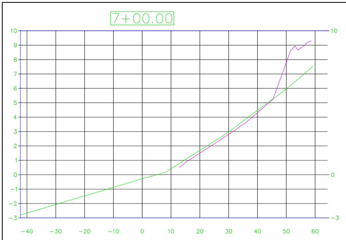
Figure 5-31 Profile 7 + 00. Green and pink lines represent November 09, 2015, and November 10, 2015, elevations respectively.
