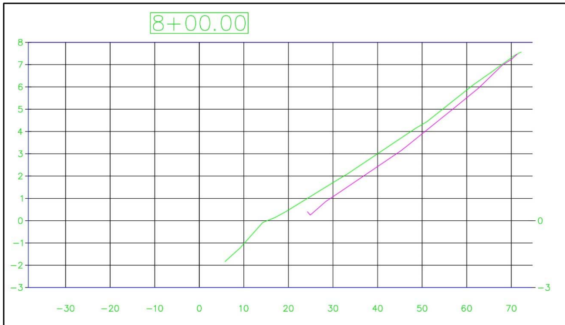
Figure 5-33 Profile 8 + 00. Green and pink lines represent November 09, 2015, and November 10, 2015, elevations respectively.
