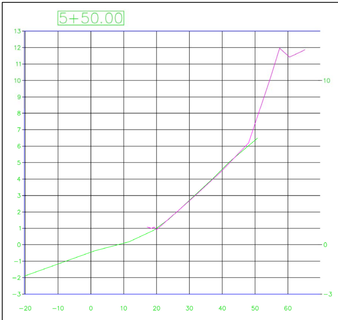
Figure 5-28 Profile 5 + 50. Green and pink lines represent November 09, 2015, and November 10, 2015, elevations respectively.
