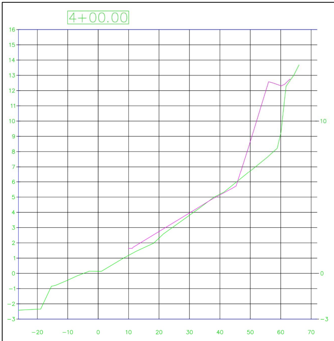
Figure 5-25 Profile 4 + 00. Green and pink lines represent November 09, 2015, and November 10, 2015, elevations respectively.
