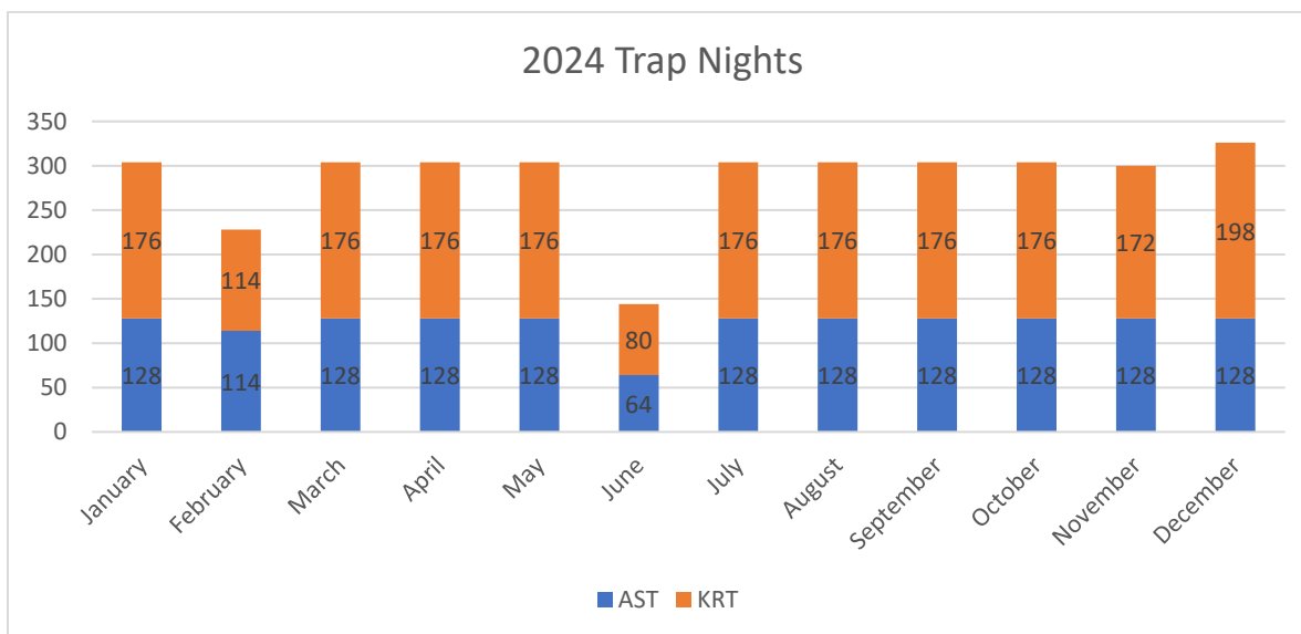
Figure 7. Number of predator trap-nights in 2024 on the Alaka'i Swamp Trail (AST) and Kalalau Rim Trail (KRT). The KSHCP prescribes a minimum of 300 trap-nights per month.
