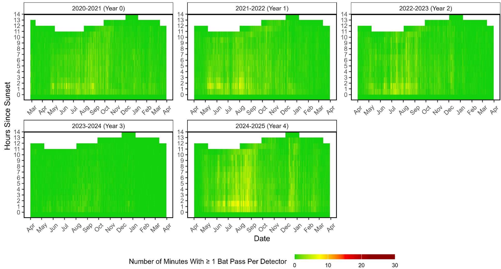
Figure 4.5. Bat activity patterns relative to sunset (hour zero), illustrated by the number of minutes with one or more bat calls averaged across acoustic sampling stations, within Auwahi Wind Energy’s Tier 4 Mitigation Site, from February 16, 2020, to March 30, 2025, Maui, Hawaii.
