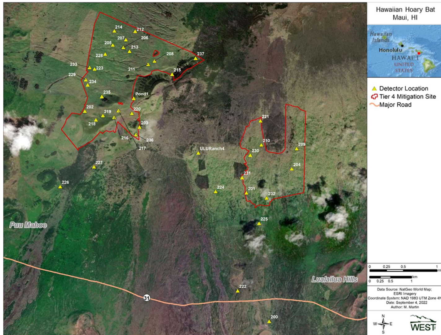
Figure 1.1. Location of Auwahi Wind Energy's Hawaiian hoary bat Tier 4 Mitigation Site and acoustic bat detector locations, Maui, Hawaii.
