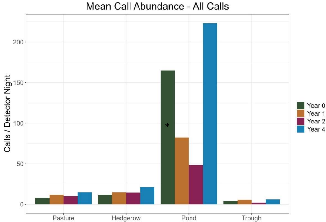
Figure 4.1. Mean number of bat calls per detector-night for all acoustic detectors, by habitat feature type and year, in Auwahi Wind Energy's Tier 4 Mitigation Site, Maui, Hawaii.
