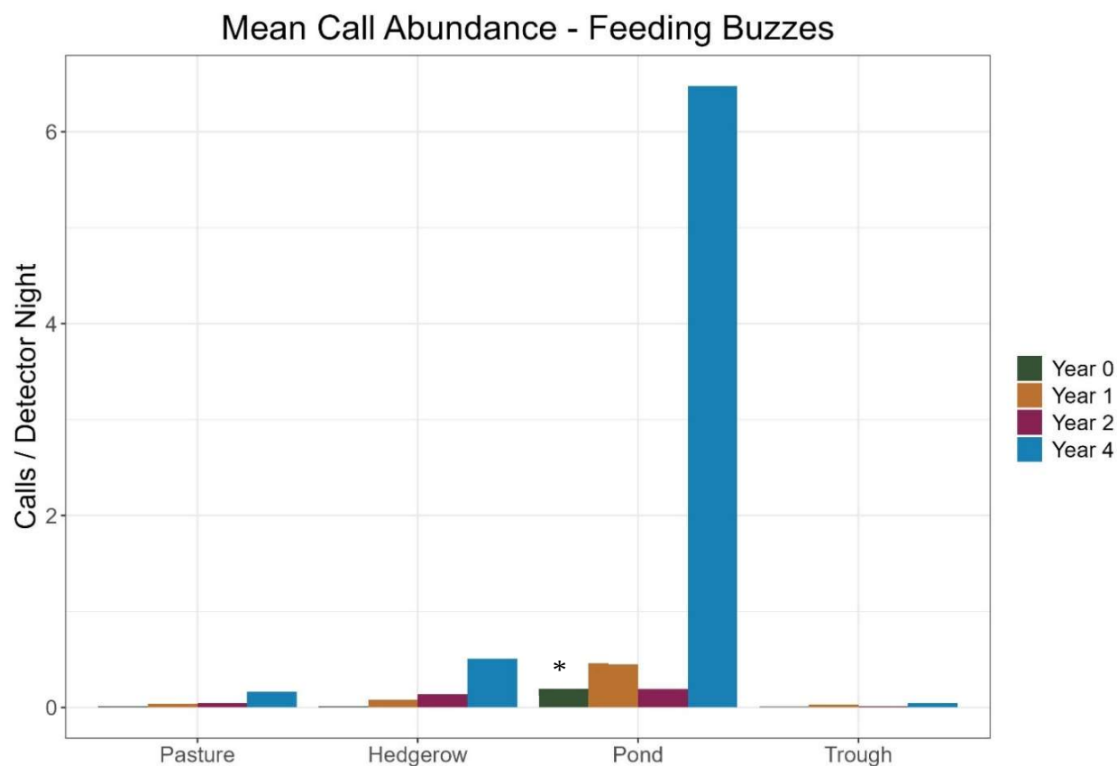
Figure 4.2. Mean number of feeding buzzes per detector-night for all acoustic detectors, by habitat feature type and year, in Auwahi Wind Energy's Tier 4 Mitigation Site, Maui, Hawaii.
