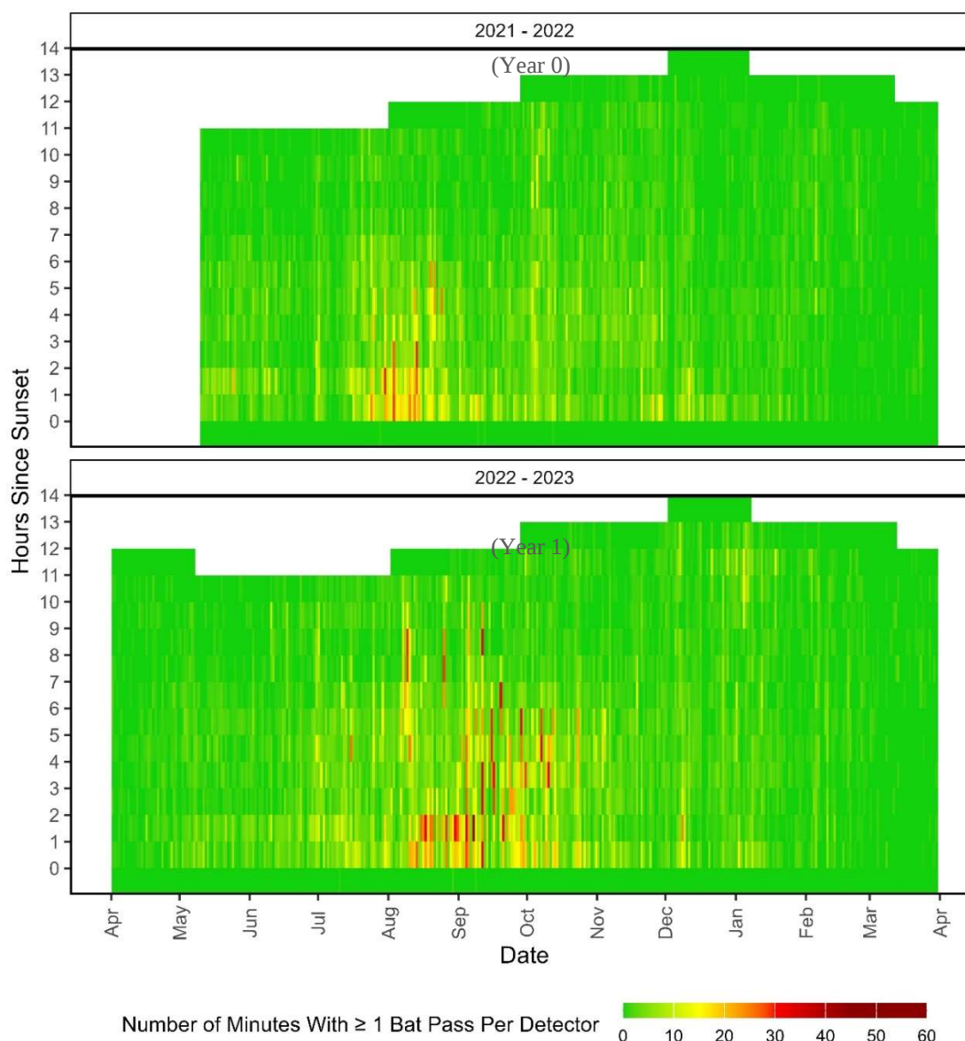
Figure 4.1. Bat activity patterns relative to sunset (hour zero) and time of year illustrated by the number of minutes with one or more bat calls averaged across the two acoustic sampling stations within Auwahi Wind's Tier 5 Mitigation Site May 11, 2021–March 31, 2023, Maui, Hawaii.
