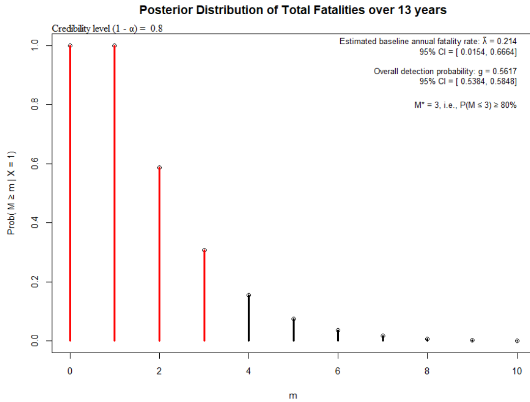
Figure 5. Evidence of Absence Total Mortality Output for Hawaiian Petrel Multi-Year Analysis in FY 2025 (Dalthorp et al. 2017)
