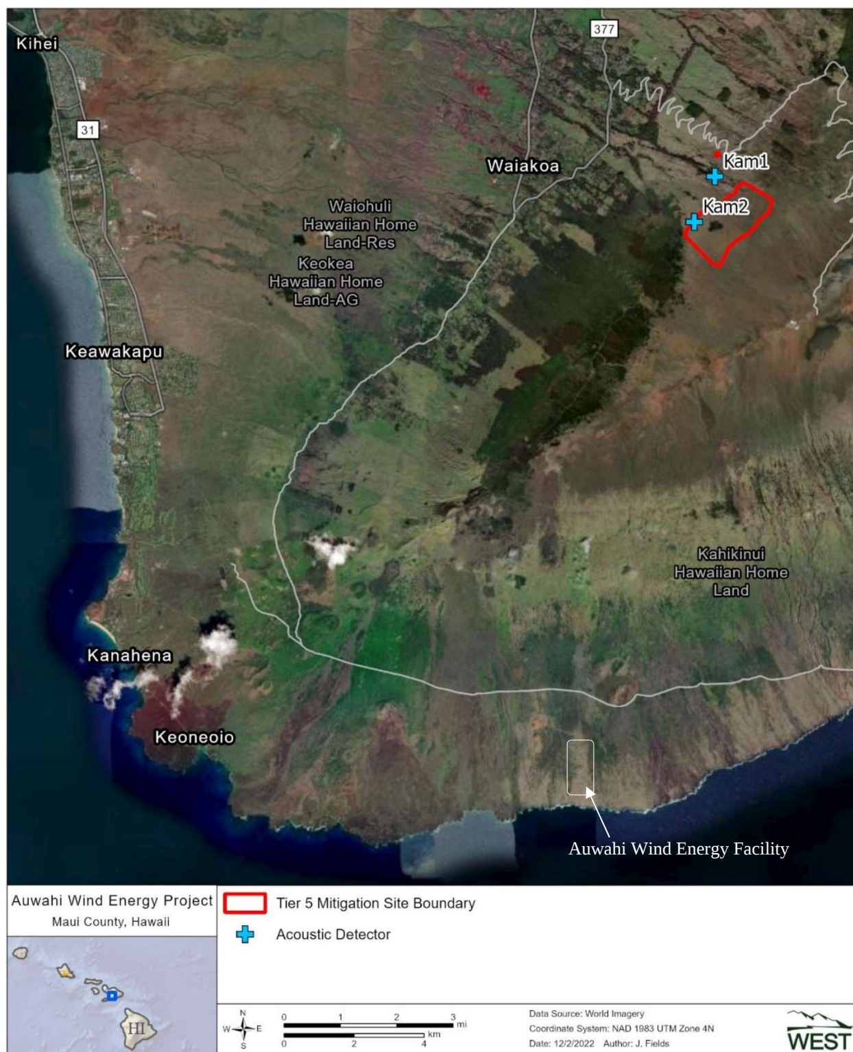
Figure 1.1. Location of Auwahi Wind Energy’s Tier 5 Hawaiian hoary bat Mitigation Site and acoustic bat detector locations, Maui, Hawaii.
