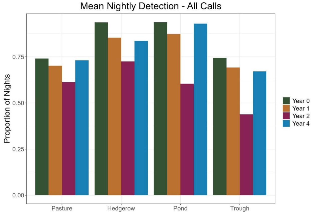
Figure 4.3. The proportion of nights with bat calls for all acoustic detectors, by habitat feature type and year, in Auwahi Wind Energy’s Tier 4 Mitigation Site, Maui, Hawaii.
