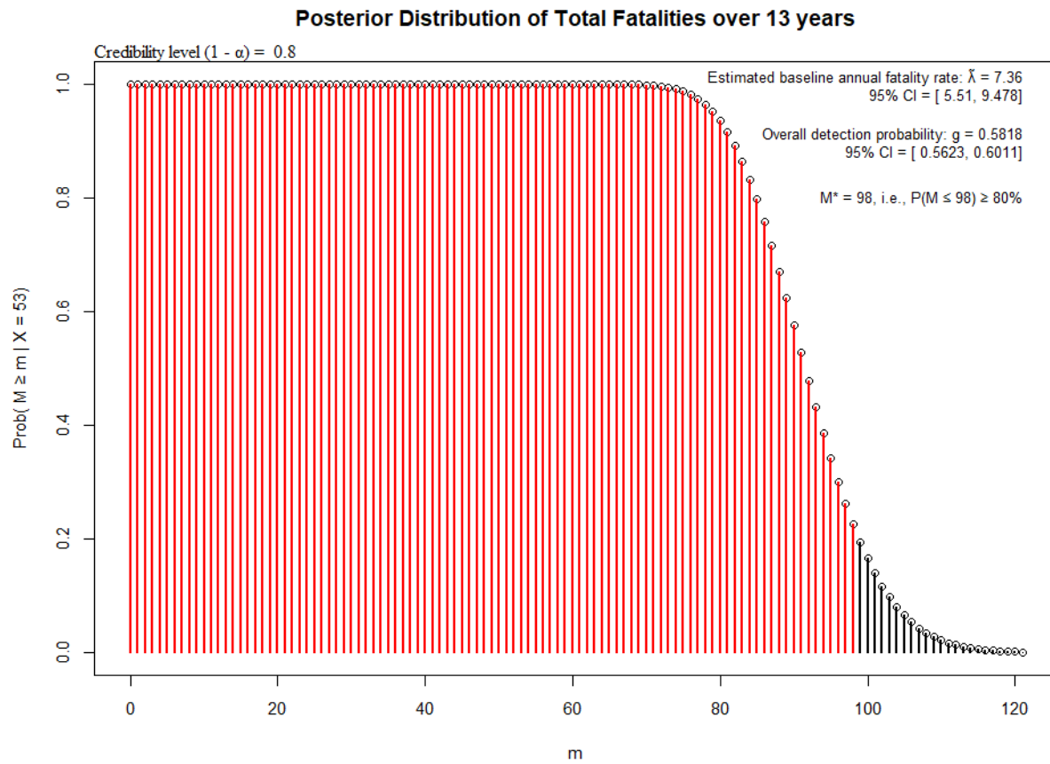
Figure 2. Evidence of Absence Total Mortality Output for Hawaiian Hoary Bat Multi-Year Analysis in FY 2025 (Dalthorp et al. 2017)
