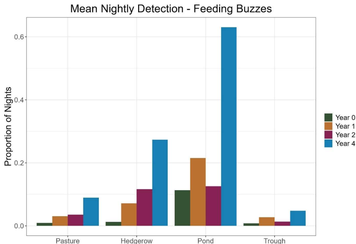
Figure 4.4. The proportion of nights with feeding buzzes for all acoustic detectors, by habitat feature type and year, in Auwahi Wind Energy's Tier 4 Mitigation Site, Maui, Hawaii.
