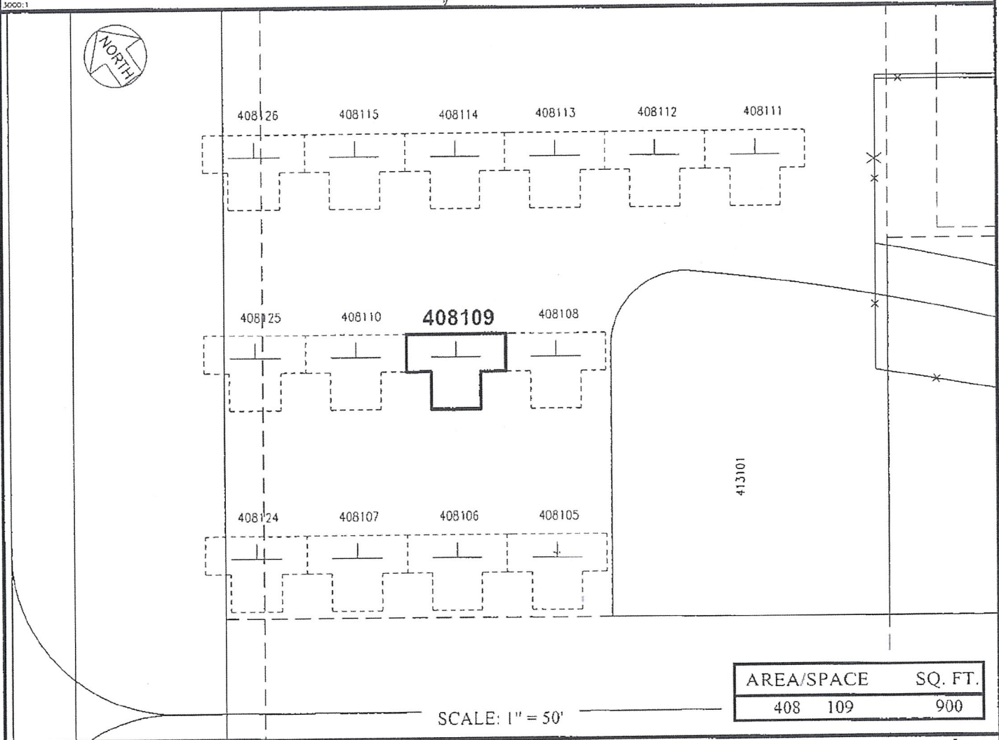
LOCATION PLAN
