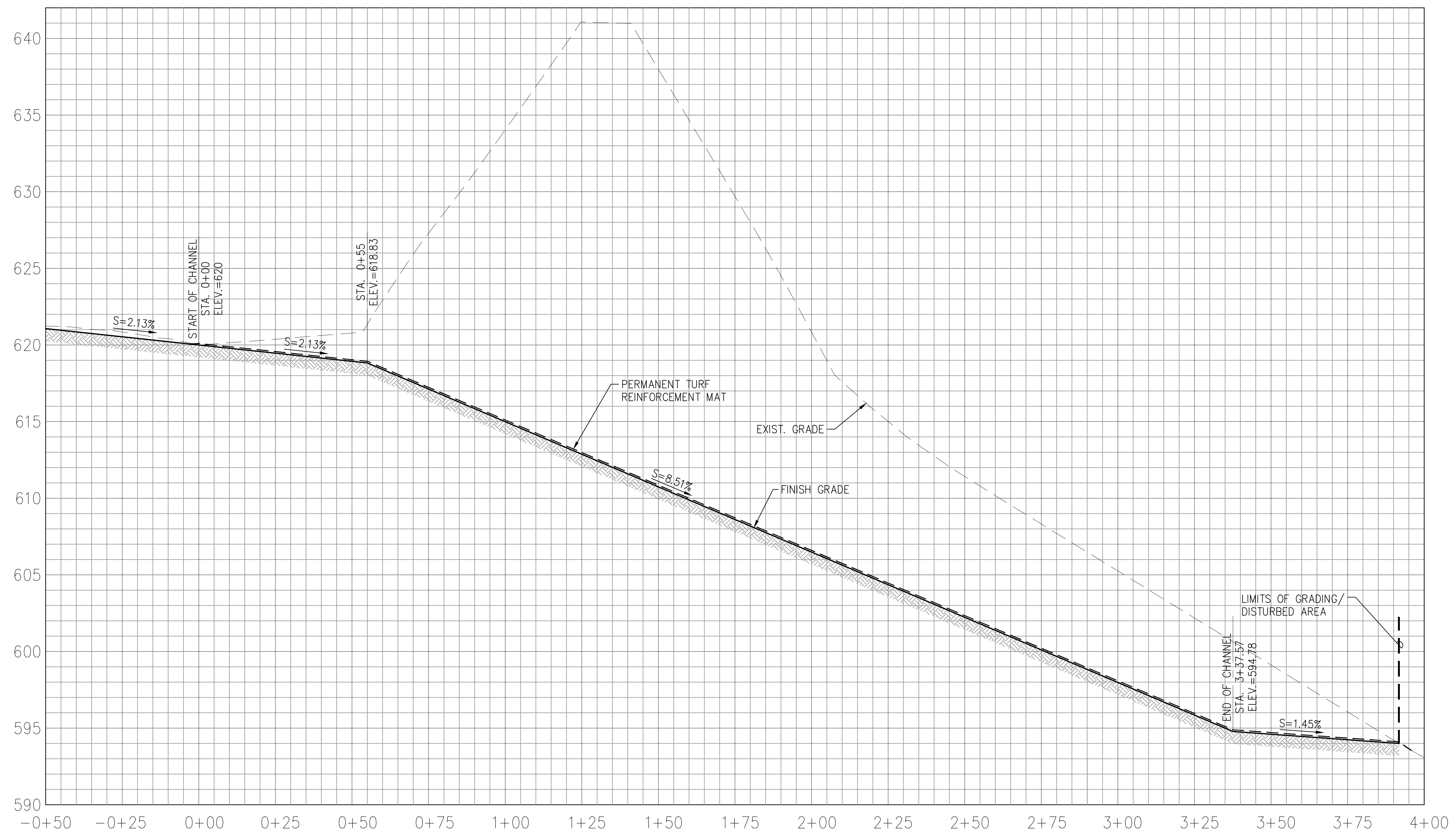
PROFILE SCALE: HOR. 1"=20'-0" VERT. 1"=4'-0"
