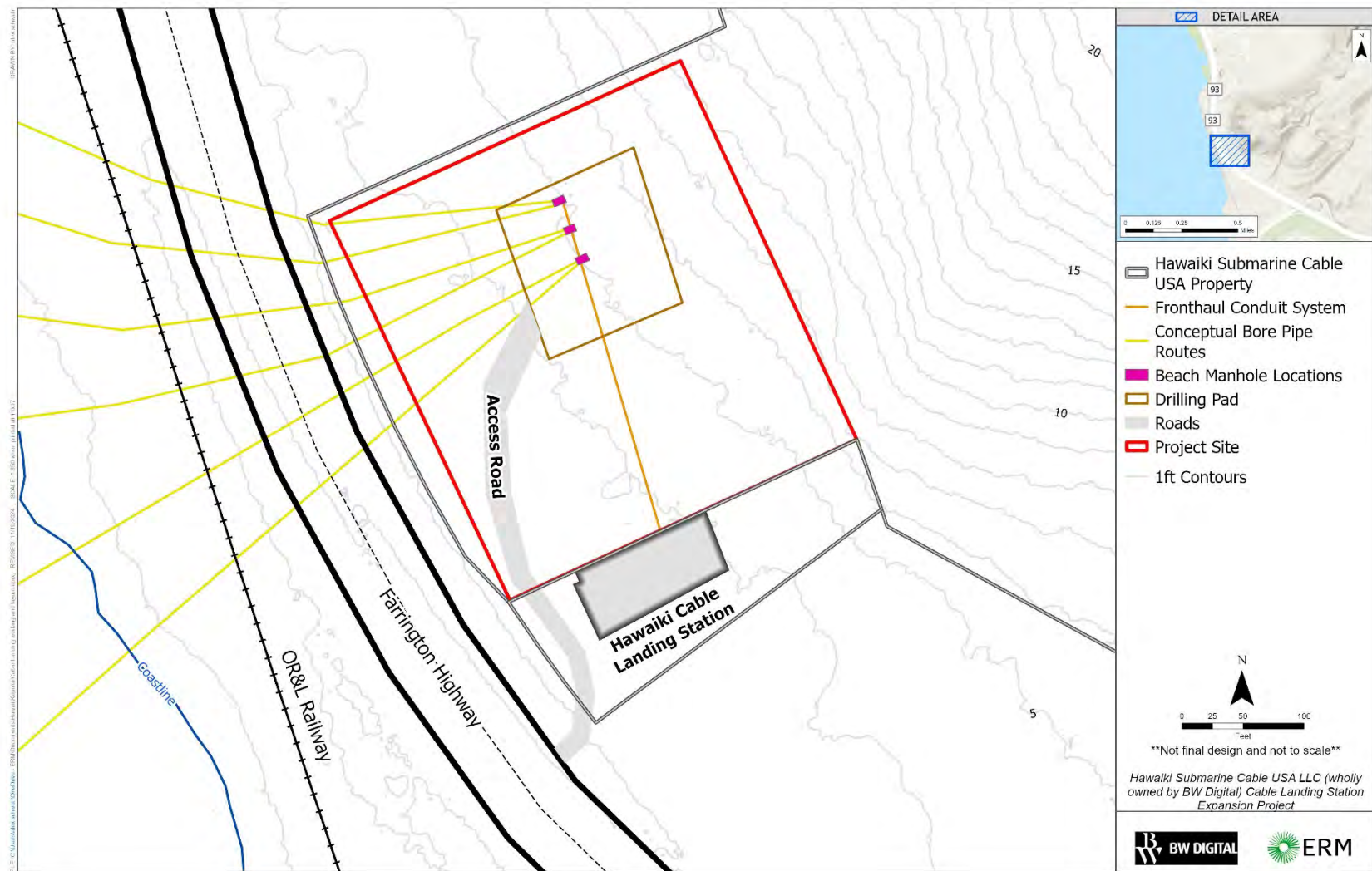
FIGURE 1-5: HDD SCHEMATIC
